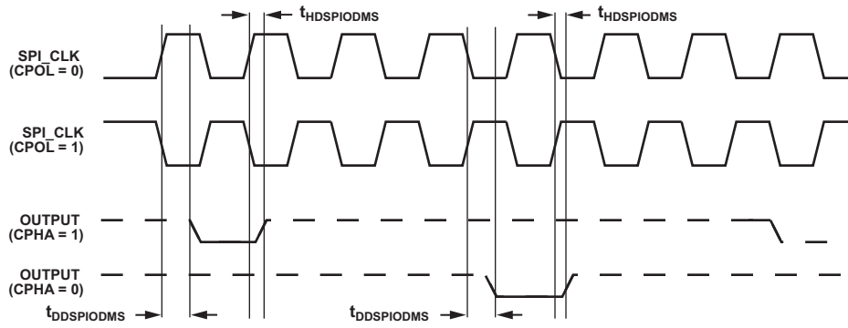
Figure 36. ODM Slave
