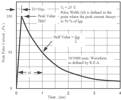
Fig. 3 Pulse Waveform
