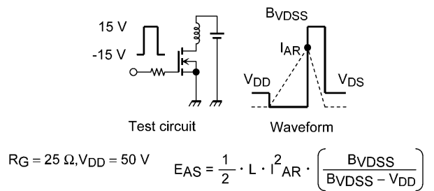
Fig. 8.16 Test Circuit/Waveform
