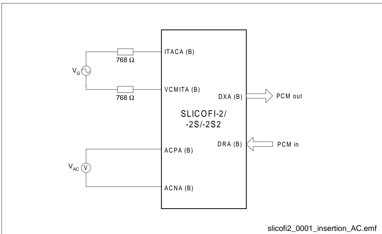
Figure 13 Insertion Loss
