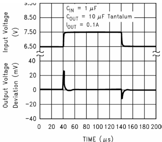
B2117-5.0 Line Transient Response
