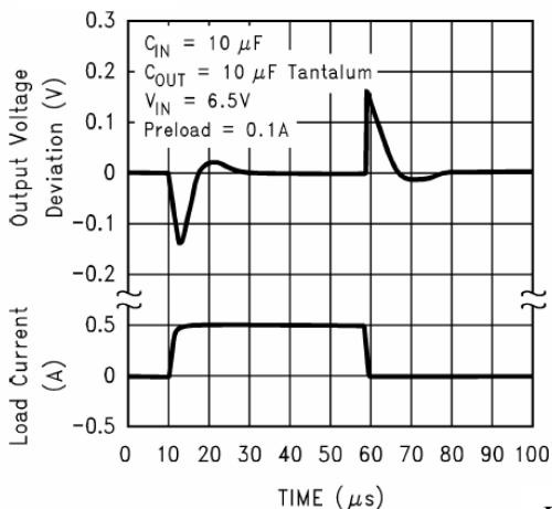
B2117-5.0 Load Transient Response
