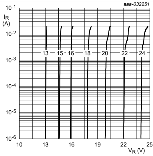
Fig. 9. Reverse current as a function of reverse voltage; typical values (MM3Z13VT1G to 24VT1G)
