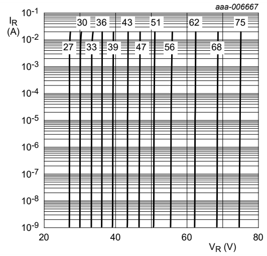
Fig. 10. Reverse current as a function of reverse voltage; typical values (MM3Z27VT1G to 75VT1G)
