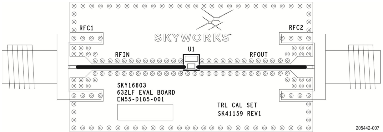
Figure 7. SKY16603-632LF Evaluation Board Assembly Diagram
