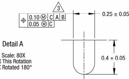
Figure 11. SKY16603-632LF Package Dimensions
