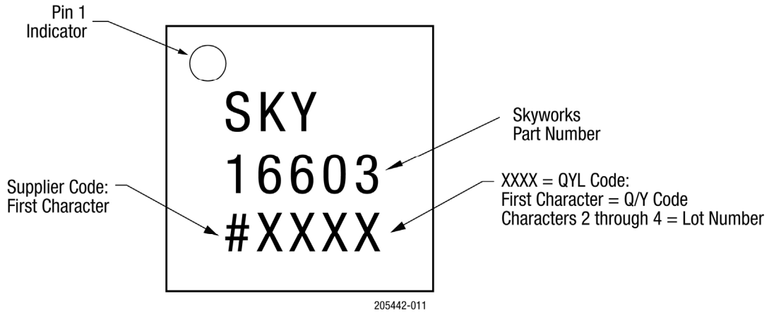
Figure 10. SKY16603-632LF Typical Part Markings
