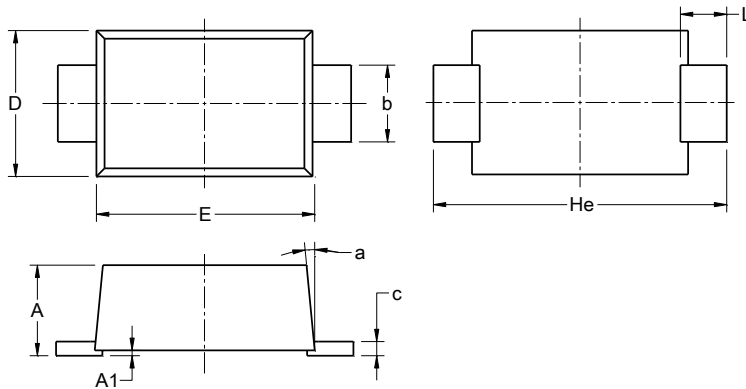
DO-219AA
