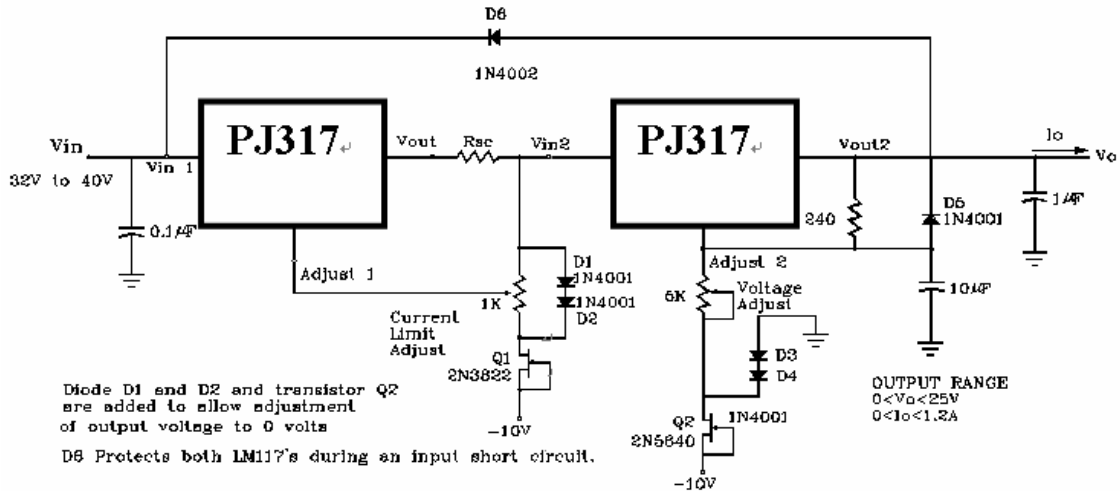
FIGURE 19 - "LABORATORY" POWER SUPPLY WITH ADJUSTABLE CURRENT LIMIT AND OUTPUT VOLTAGE
