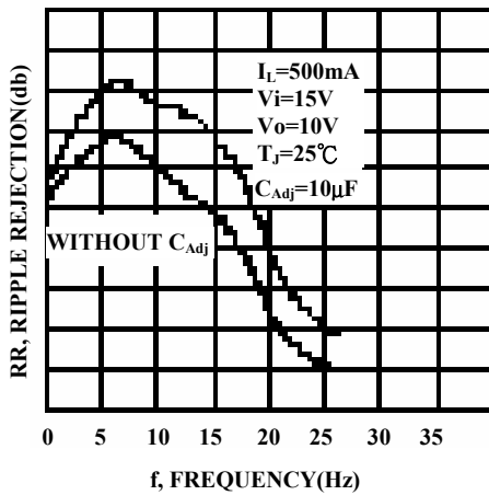
FIGURE 13-RIPPLE REJECTION versus FREQUENCY
