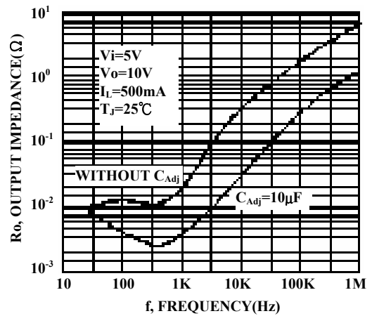
FIGURE 14-OUTPUT IMPEDANCE
