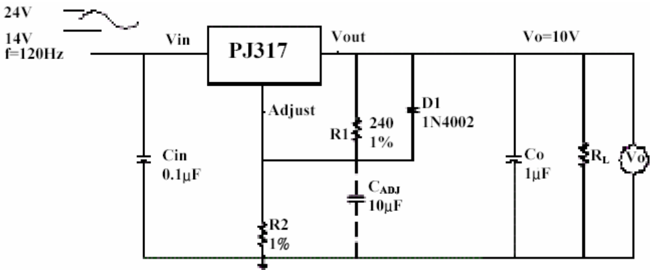
FIGURE 4 – RIPPLE REJECTION TEST CIRCUIT
