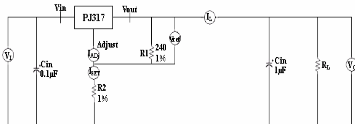
FIGURE 3 – STANDARD TEST CIRCUIT
