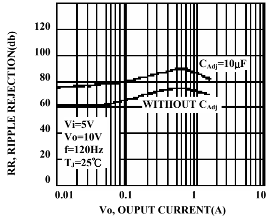
FIGURE 12-RIPPLE REJECTION versus OUTPUT CURRENT
