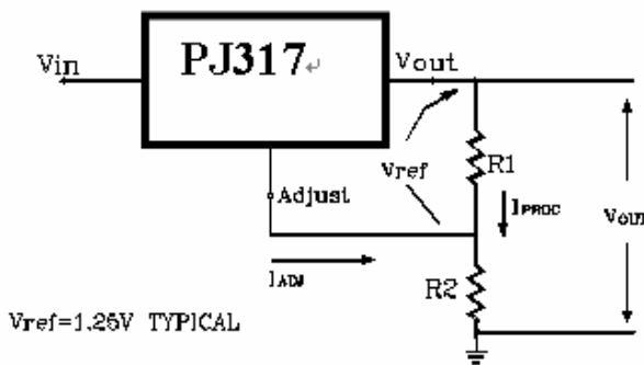
FIGURE 17 – BASIC CIRCUIT CONFIGURATION
