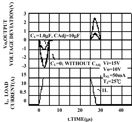
FIGURE 16-LOAD TRANSIENT RESPONSE
