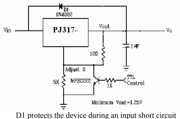
FIGURE 21 - 5V ELECTRONIC SHUT DOWN REGULATOR
