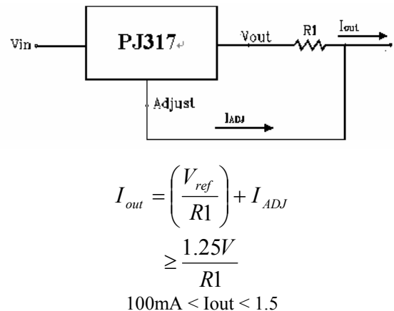
FIGURE 23 - CURRENT REGULATOR
