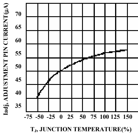
FIGURE 7-ADJUSTMENT PIN CURRENT
