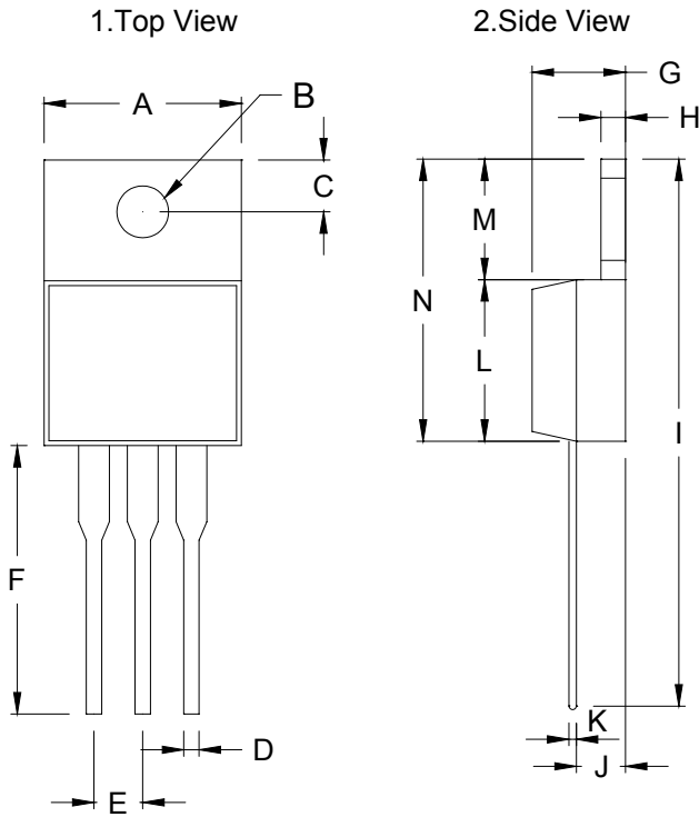
TO-220 Mechanical drawing
