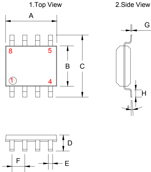
SOP-8 Mechanical drawing
