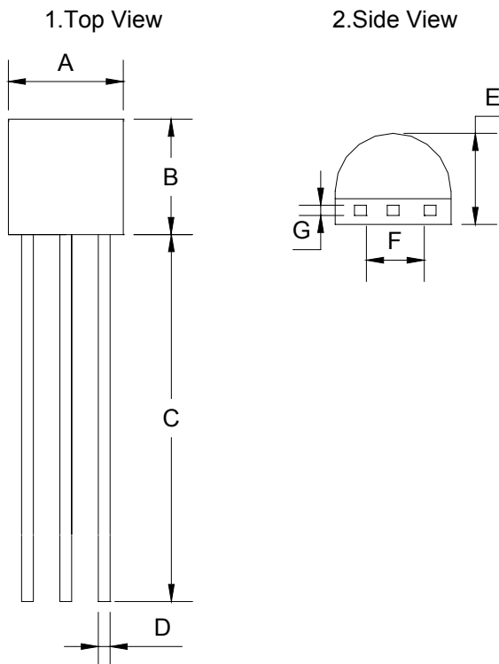
TO-92 Mechanical drawing
