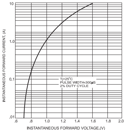
FIG.3- TYPICAL INSTANTANEOUS FORWARD CHARACTERISTICS PER BRIDGE ELEMENT
