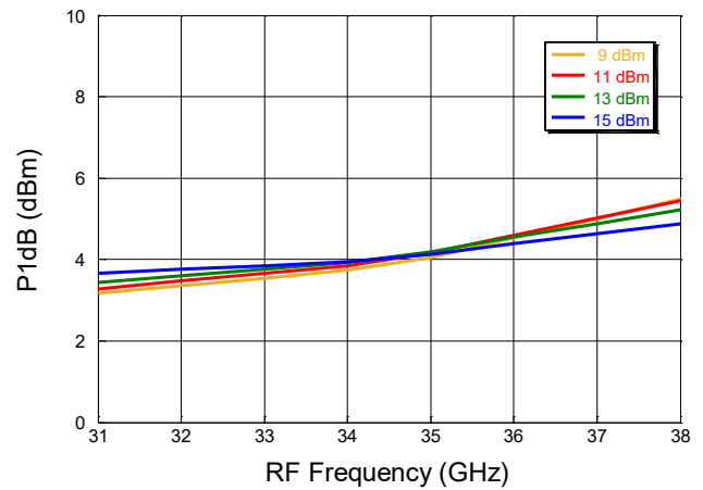
P1dB over LO drive vs. RF Frequency
