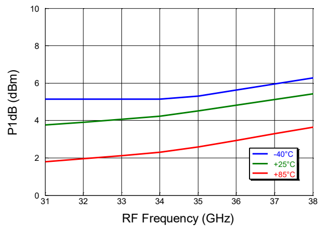
P1dB vs. RF Frequency (Up Conversion)
