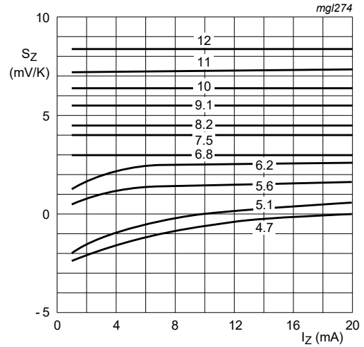
Fig. 6. Temperature coefficient as a function of working current; typical values (SZMM3Z4V7T1G to 12V1G)
