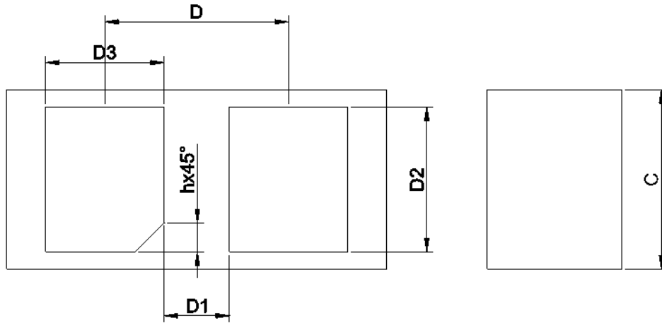
DFN0603-2L
