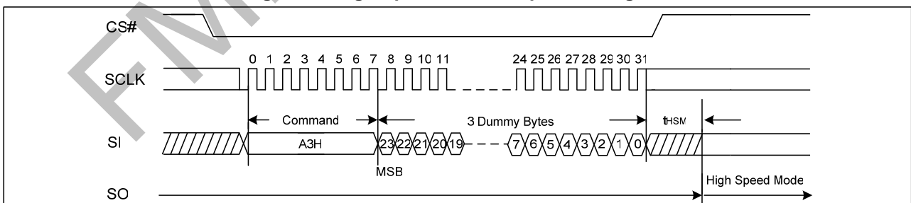
Figure28. High Speed mode Sequence Diagram
