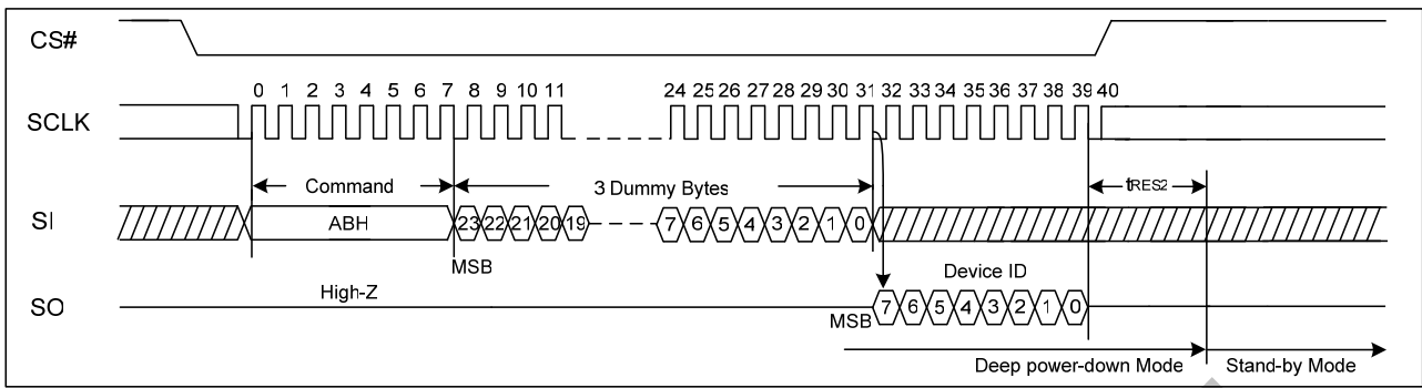
Figure25. Release Power-Down/Read Device ID Sequence Diagram
