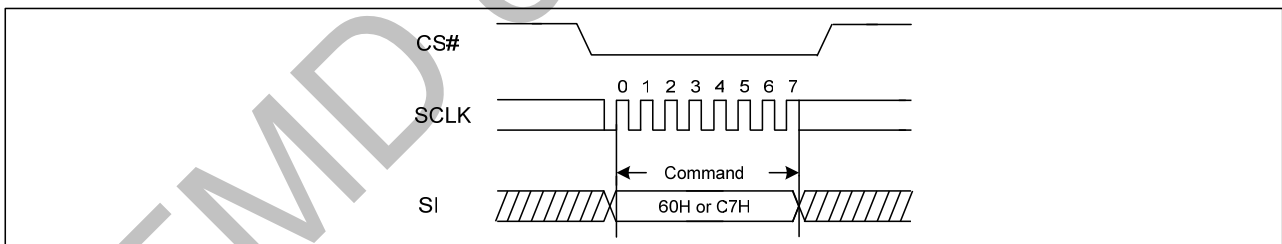
Figure22. Chip Erase Sequence Diagram
