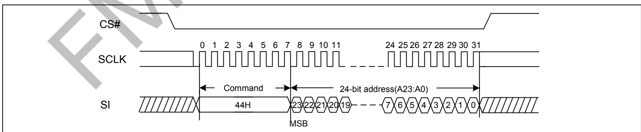
Figure32. Erase Security Registers command Sequence Diagram
