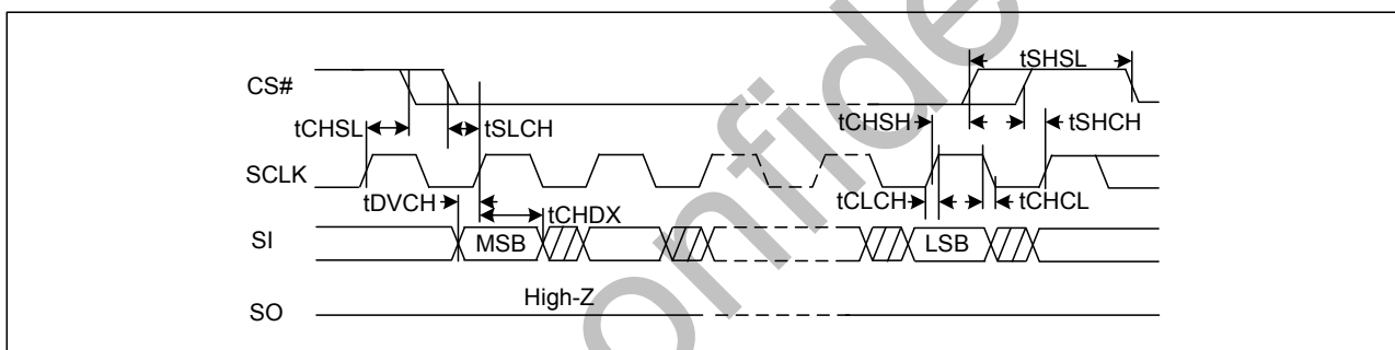
Figure38. Output Timing
