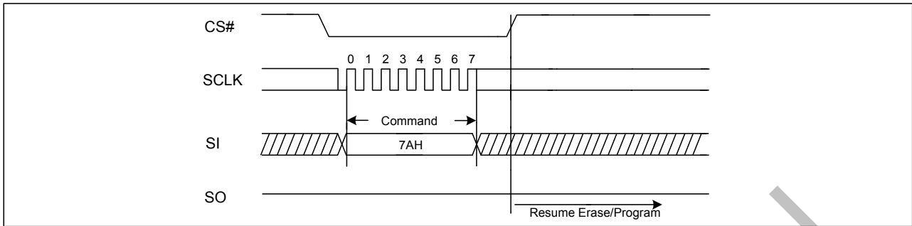
Figure31. Program/Erase Resume Sequence Diagram
