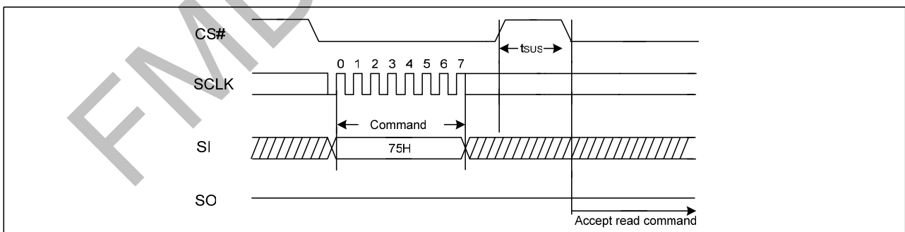
Figure30. Program/Erase Suspend Sequence Diagram
