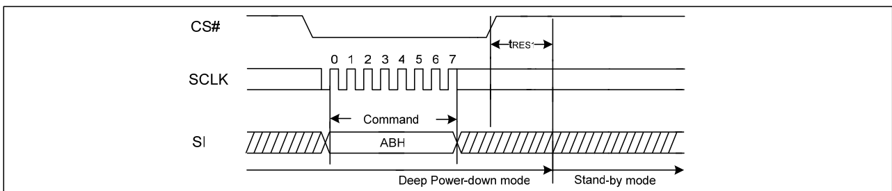
Figure24. Release Power-Down Sequence Diagram
