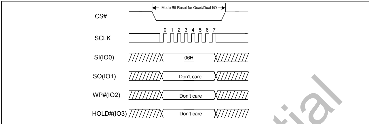
Figure29. Continuous Read Mode Reset Sequence Diagram
