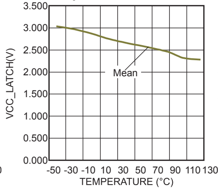
VCC_Latch vs. Temperature Chart
