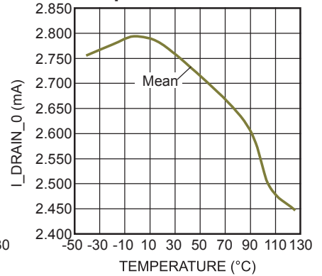
I_DRAIN_0 vs. Temperature Chart
