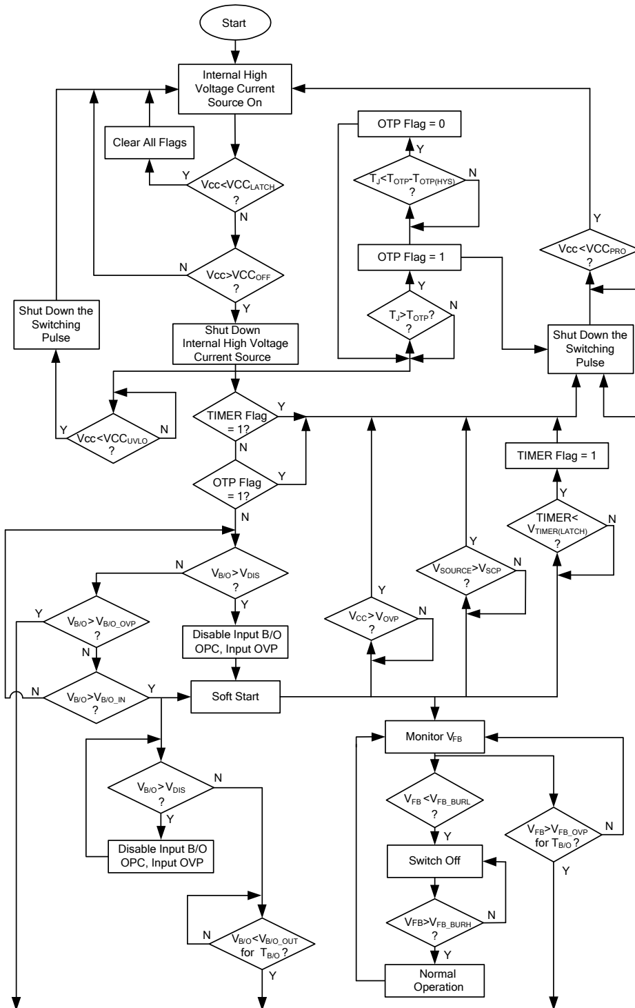
Figure 15: Flow Chart
