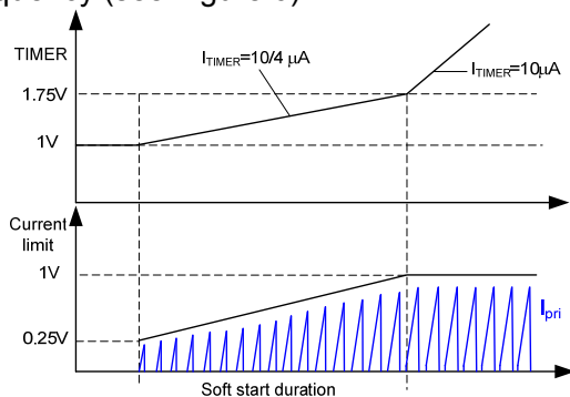
Figure 6: Soft Start
