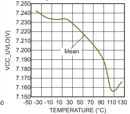
VCC_UVLO vs. Temperature Chart
