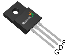
TO-220FP
