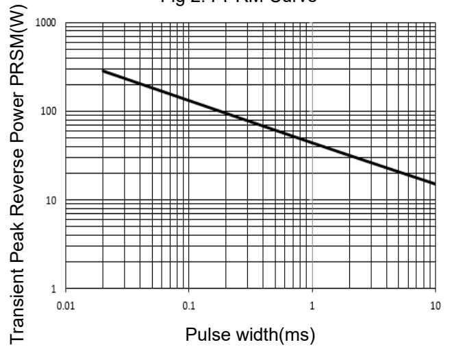
Fig 2. PPRM Curve
