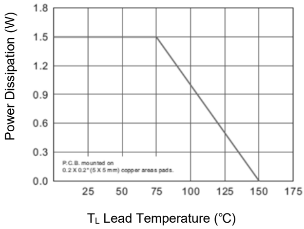
Fig 1. Maximum Continuous Power Derating
