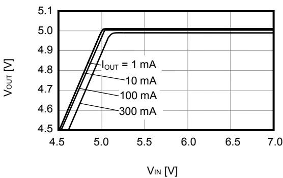
S-1170B50 (Ta=25°C)
