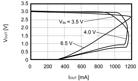
S-1170B30 (Ta=25°C)
