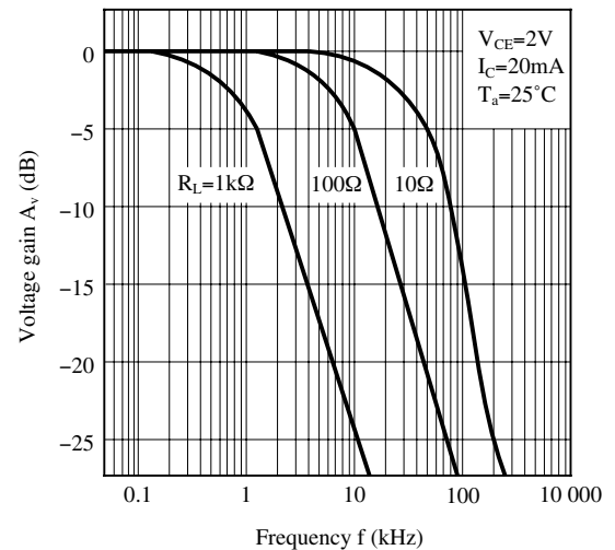
Fig.12 Frequency Response
