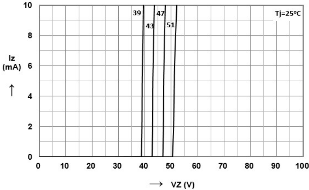
BREAKDOWN CHARACTERISTICS at T_j=\text{constant} (pulsed)
