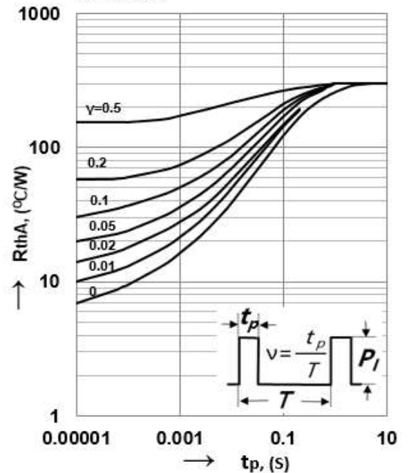
Pulse thermal resistance versus pulse duration Valid provided that leads are kept at ambient temperature
