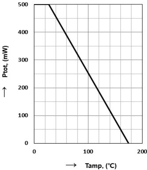
Admissible power dissipation versus ambient temperature Valid provided that leads are kept at ambient temperature
