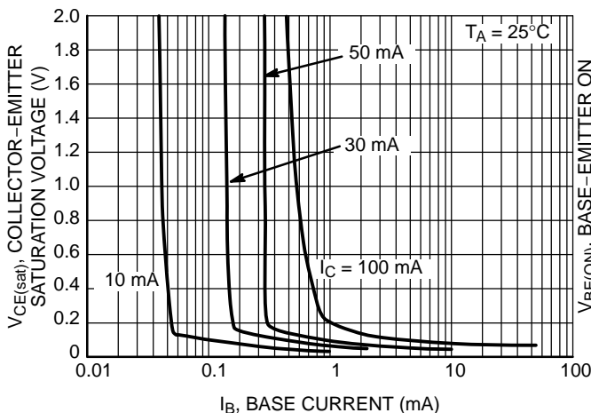
Figure 5. Saturation Region
