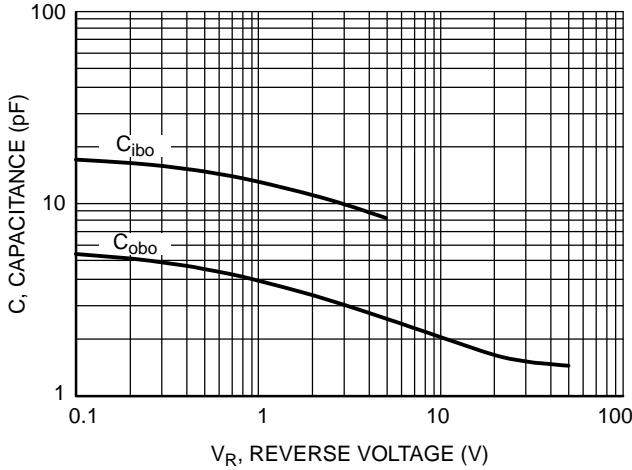
Figure 7. Capacitance
