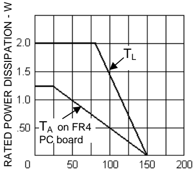
Rated Power Dissipation - W T_L , LEAD TEMP. (°C) or T_A on FR4 PC Board FIGURE 1 Power Derating Curve
