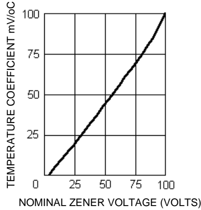
TEMPERATURE COEFFICIENT mV/°C NOMINAL ZENER VOLTAGE (VOLTS) FIGURE 2 Temp. Coeff. vs. Zener Voltage
