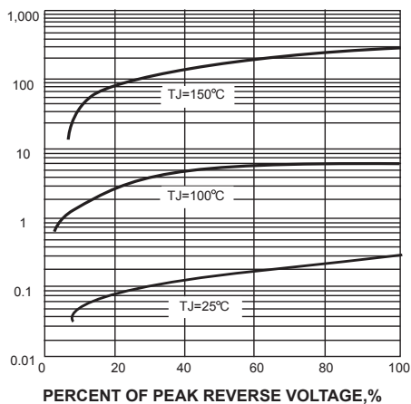
FIG. 4-TYPICAL REVERSE CHARACTERISTICS
