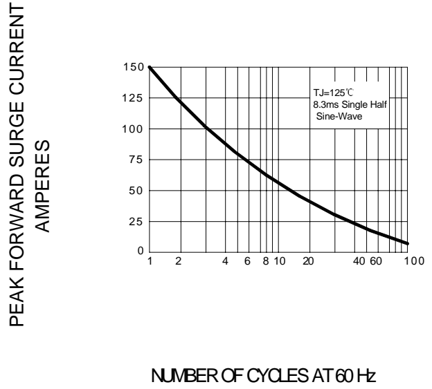
FIG.2- FORWARD SURGE CURRENT
