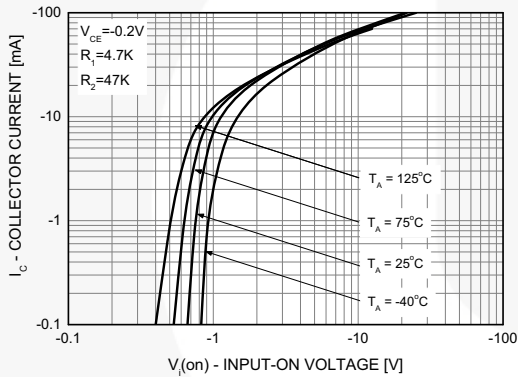
Figure 3. Input-On Voltage
