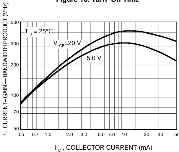
I_C , COLLECTOR CURRENT (mA) Figure 12. Current-Gain — Bandwidth Product
