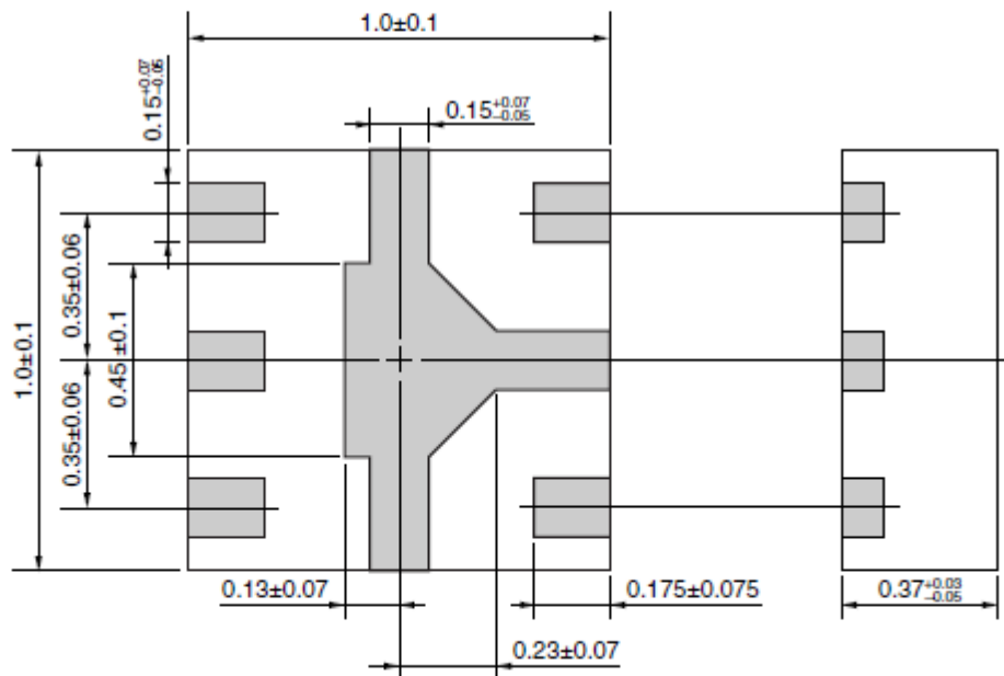
(Bottom View)
