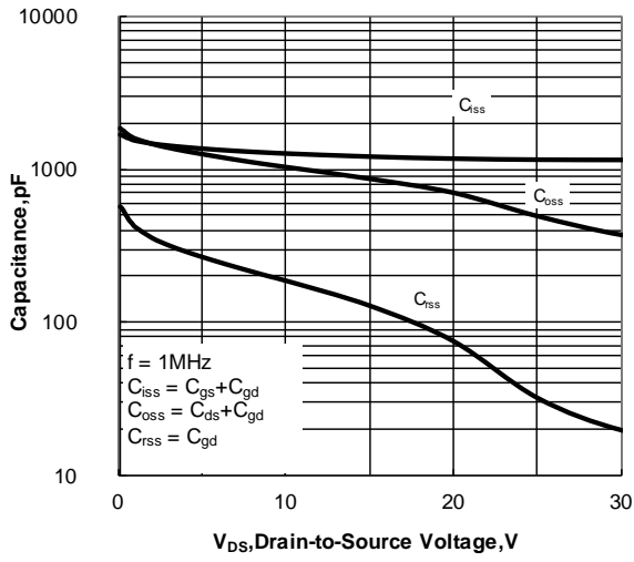
Figure 12. Capacitance Characteristics
