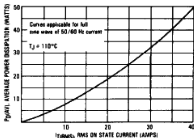
FIGURE 5 — ON-STATE POWER DISSIPATION
