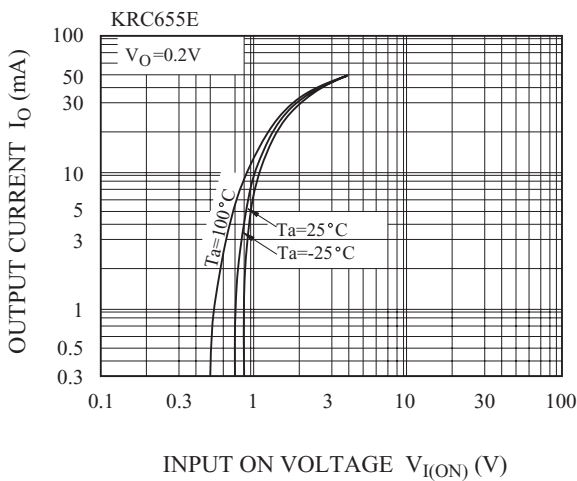
I_O - V_{I(ON)}
