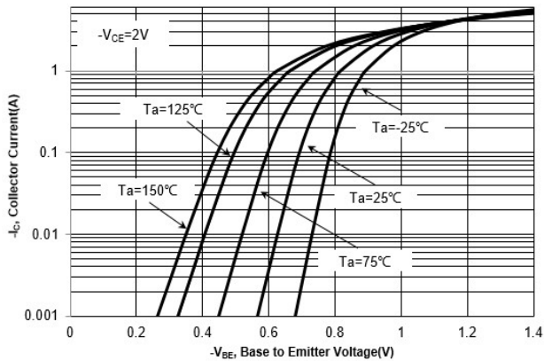
Fig. 3 Collector Current vs. Base-Emitter Voltage
