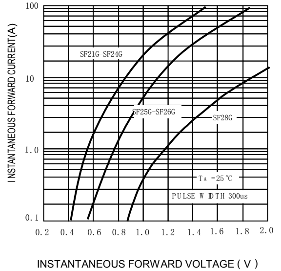
FIG.2-TYPICAL FORWARD CHARACTERISTICS
