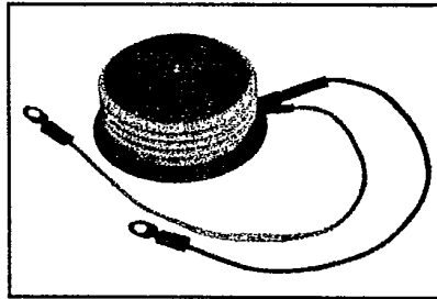
T820 Phase Control SCR 500-600 Amperes/2200-4200 Volts
