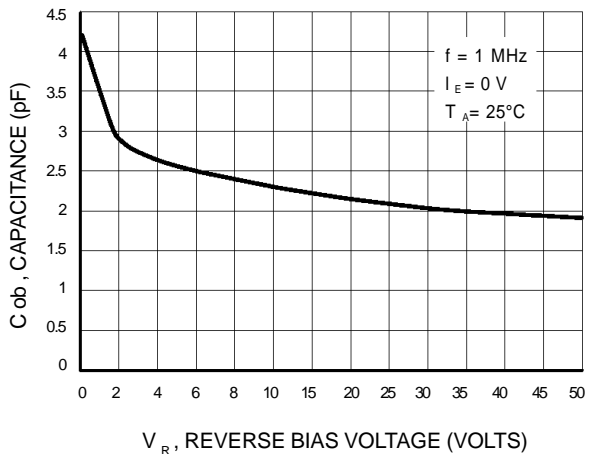
Figure 19. Output Capacitance
