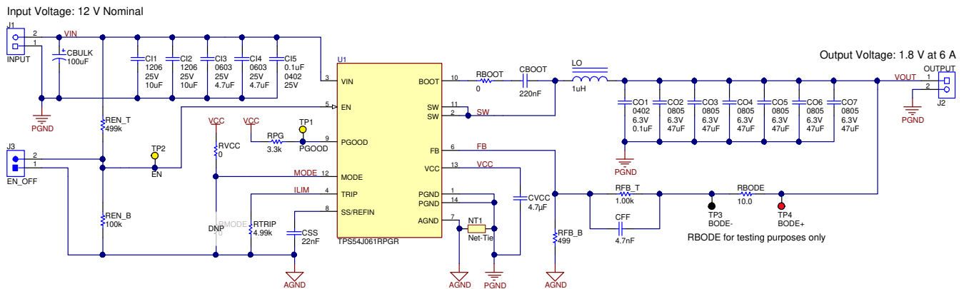
图 8-1. Application Circuit Diagram
