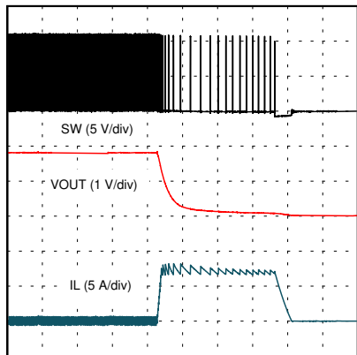
图 8-28. Overcurrent Response
