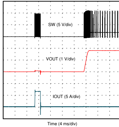
图 8-32. Overcurrent Exit Hiccup
