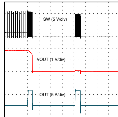
图 8-29. Overcurrent Response
