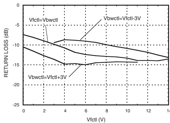
Maximum Return Loss in a 2 dB Bandwidth vs. Bandwidth Control
