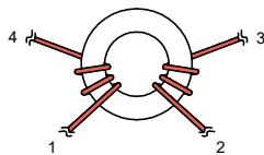
Winding Construction
