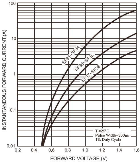
FIG.3-TYPICAL FORWARD CHARACTERISTICS
