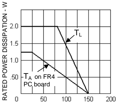
T_L , LEAD TEMP. (°C) or T_A on FR4 PC Board
