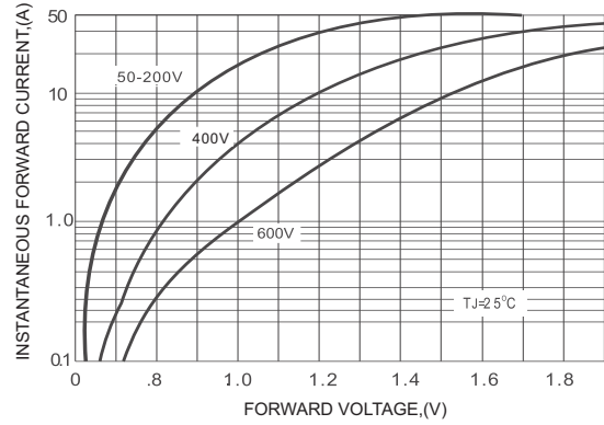
FIG.2-TYPICAL FORWARD CHARACTERISTICS
