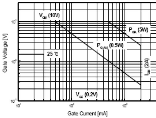
Fig1. Gate Characteristics
