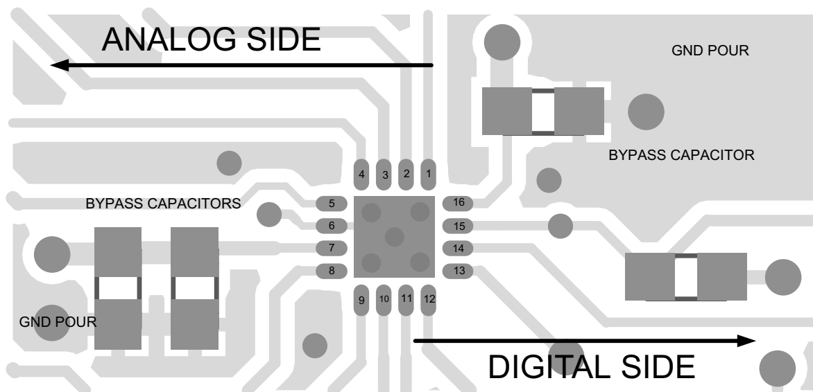
Figure 77. DACx0508 Layout Example
