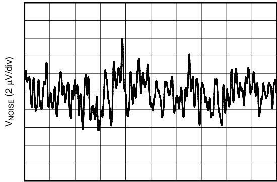
Gain = 1. External Reference = 2.5 V. DAC code at midscale
