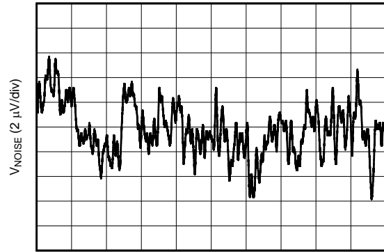
Gain = 1. DAC code at midscale
