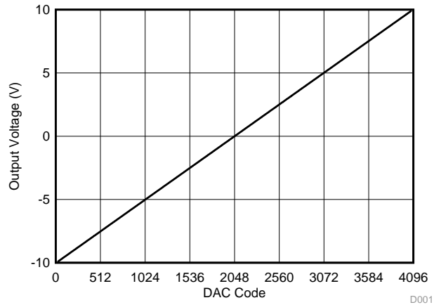
Figure 76. Bipolar Operation
