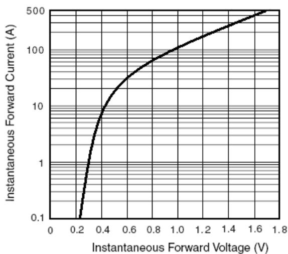
Figure 3. Typical Instantaneous Forward Characteristics Per Diode
