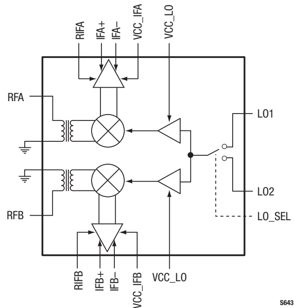
Figure 1. SKY73086-11 Block Diagram
