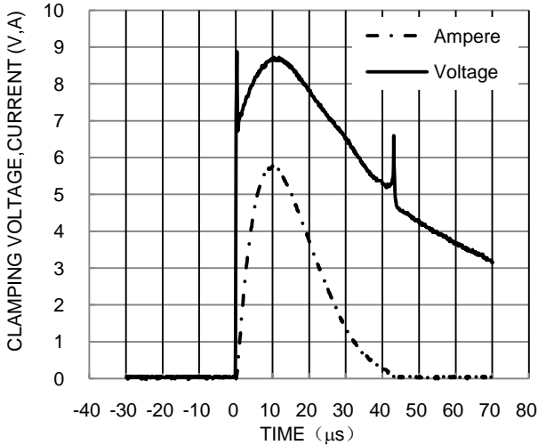
Figure 3. Waveform of Clamping Voltage, Current vs. Time (8/20µs, I/O to Vss)
