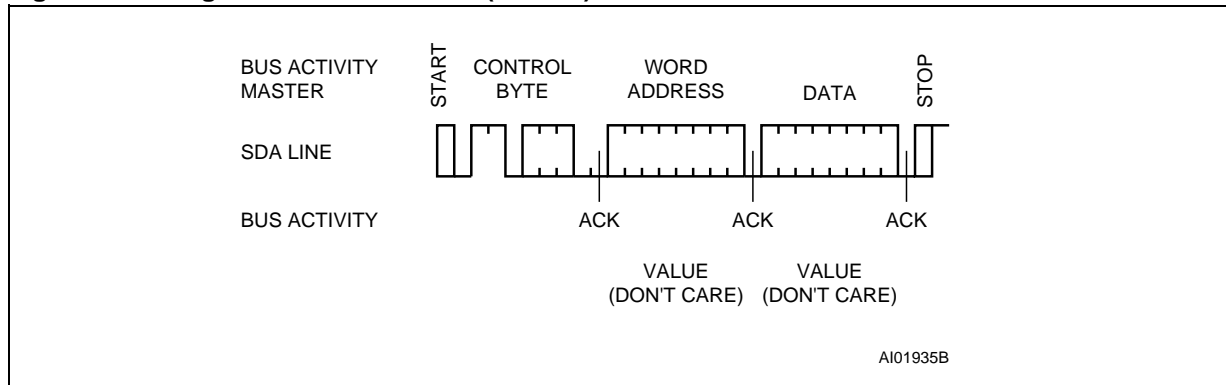
Figure 7. Setting the Write Protection ( \overline{WC} = 0 )
