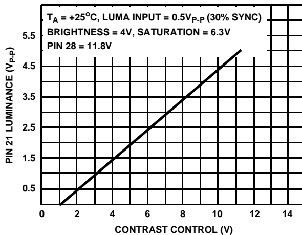
FIGURE 3. TYPICAL P 21 LUMINANCE OUTPUT vs CONTRAST CONTROL
