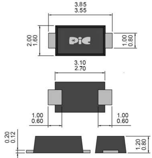
SOD-123FL
