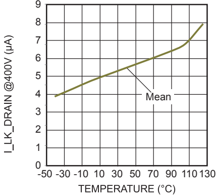
I_LK_DRAIN @400V vs. Temperature Chart
