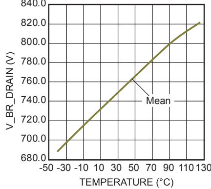
V_BR_DRAIN vs. Temperature Chart
