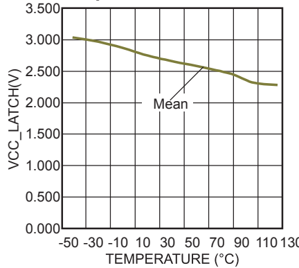
VCC_Latch vs. Temperature Chart
