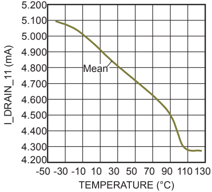
I_DRAIN_11 vs. Temperature Chart
