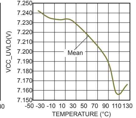
VCC_UVLO vs. Temperature Chart
