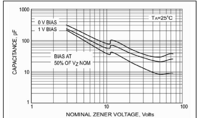
Fig.4 TYPICAL CAPACITANCE
